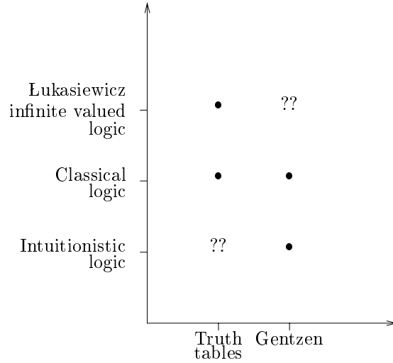
Figure 4. Logics landscape
